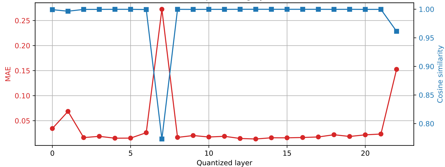
SmolLM2-1.7B-Instruct | Prompt 4 Final RMSNorm output damage | float64 \rightarrow int8
