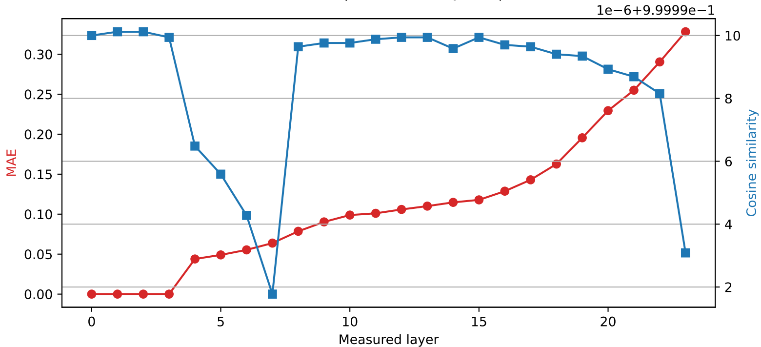
SmolLM2-1.7B-Instruct | Quantized layer 3 | float64 → int8
