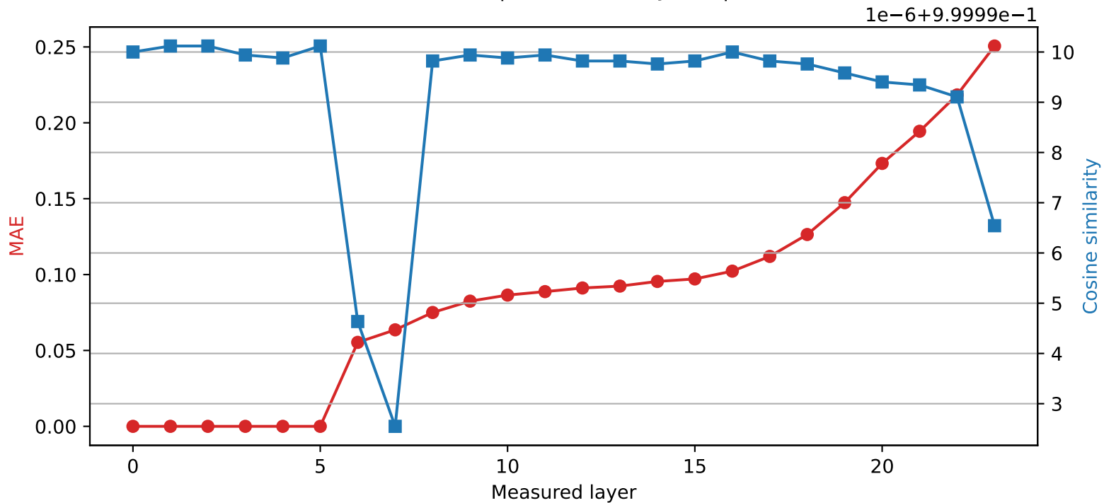
SmolLM2-1.7B-Instruct | Quantized layer 5 | float64 → int8
