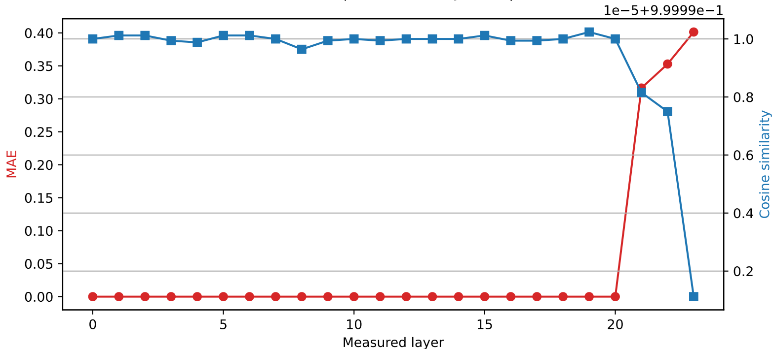
SmolLM2-1.7B-Instruct | Quantized layer 20 | float64 → int8
