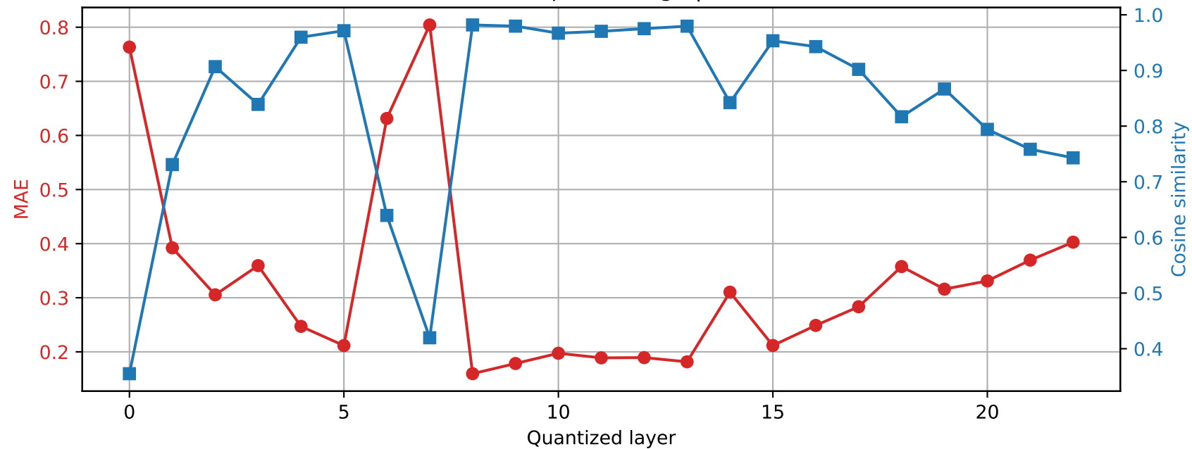
SmolLM2-1.7B-Instruct | Prompt 0 Final RMSNorm output damage | float64 \rightarrow int4
