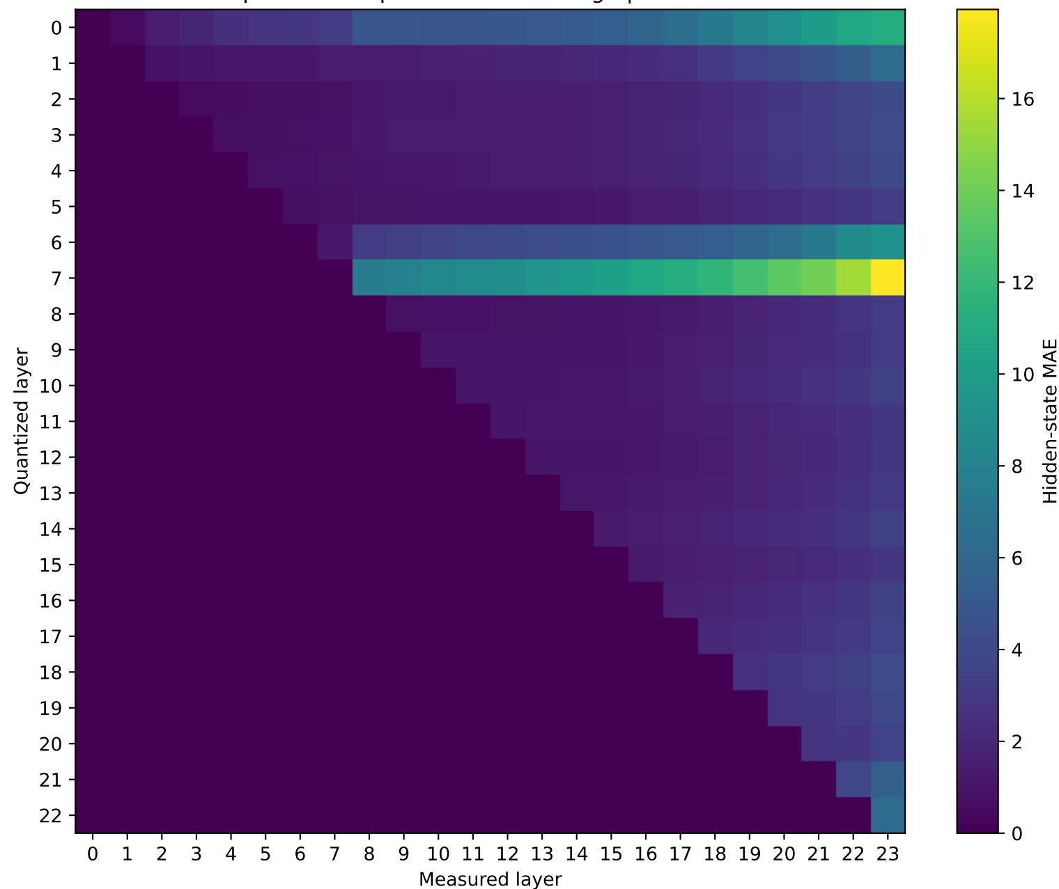
SmolLM2-1.7B-Instruct Prompt 0: MAE representation damage | float64 → int4
