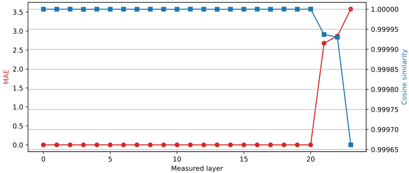
SmolLM2-1.7B-Instruct | Quantized layer 20 | float64 → int4
