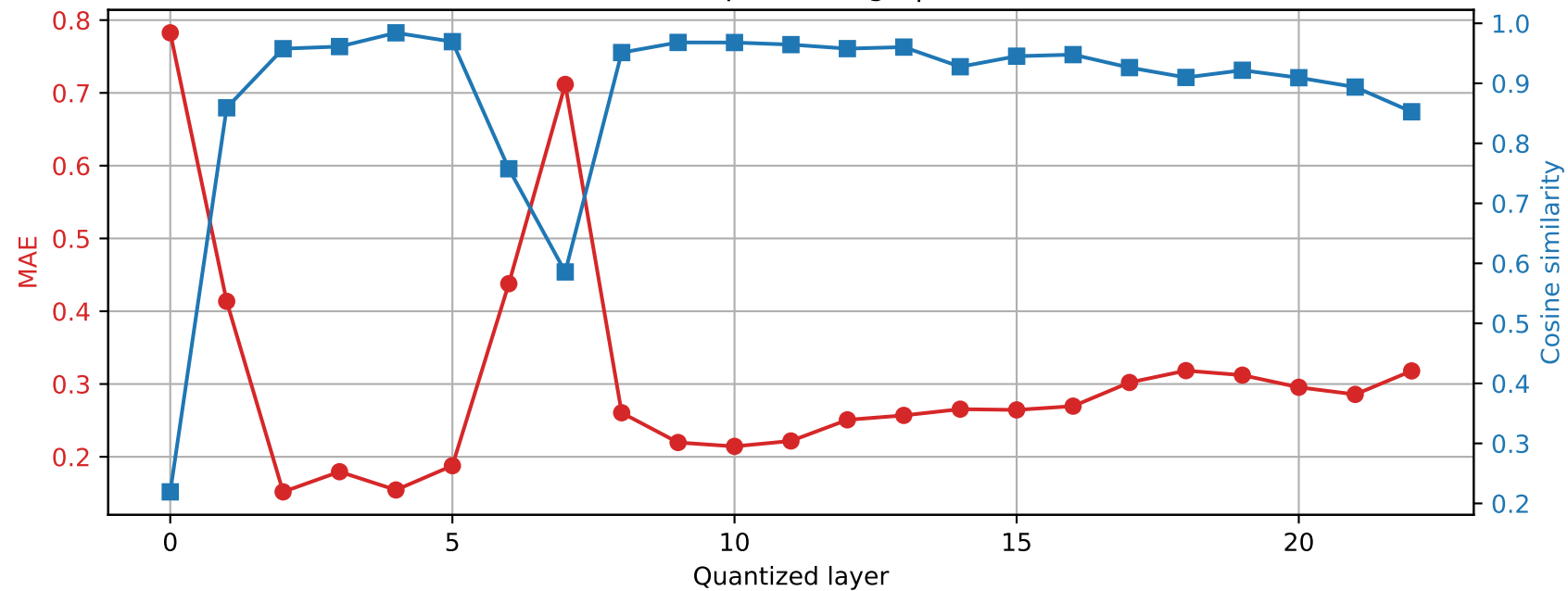
SmolLM2-1.7B-Instruct | Prompt 1 Final RMSNorm output damage | float64 \rightarrow int4
