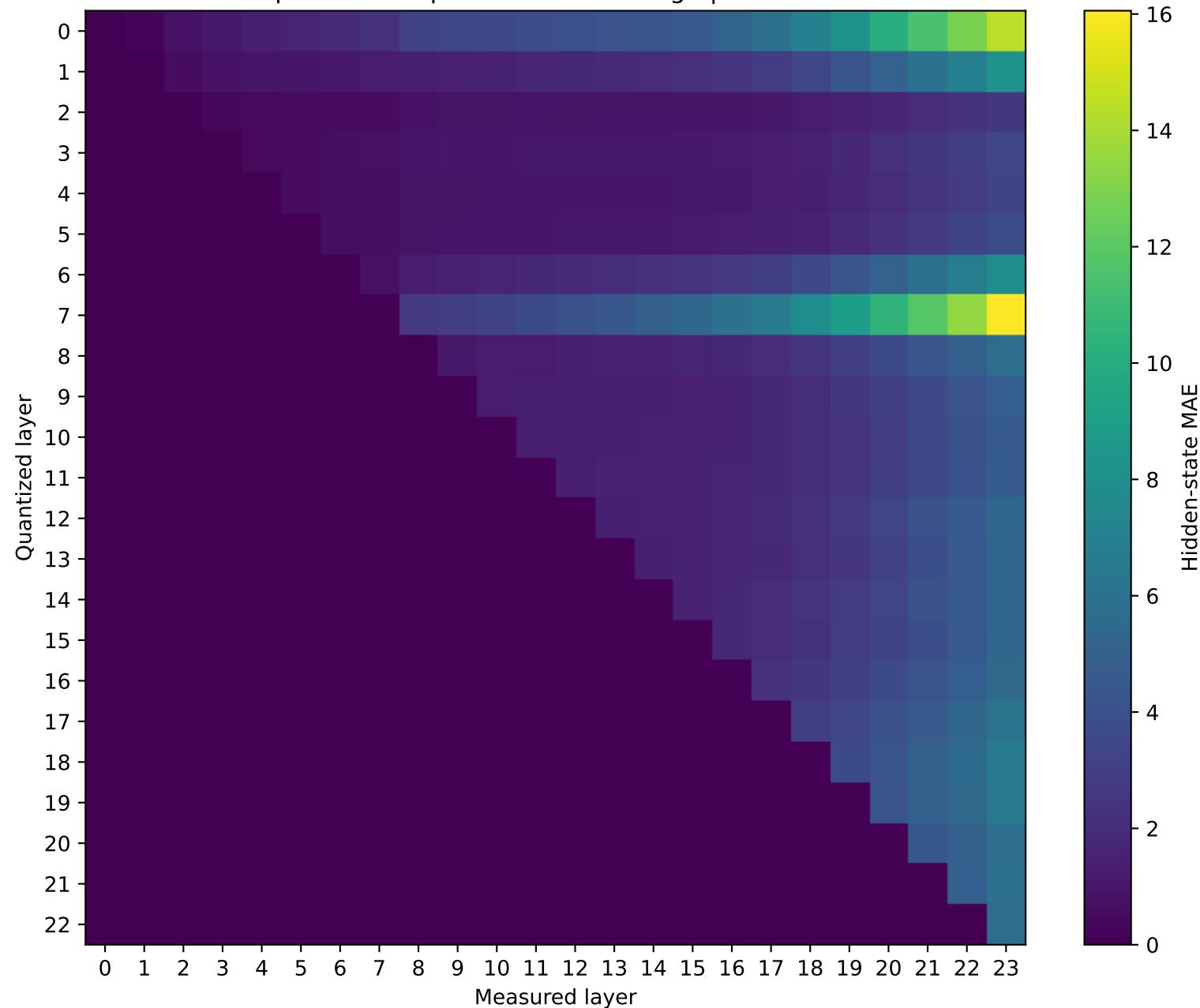
SmolLM2-1.7B-Instruct Prompt 1: MAE representation damage | float64 → int4
