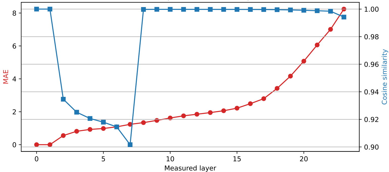
SmolLM2-1.7B-Instruct | Quantized layer 1 | float64 → int4
