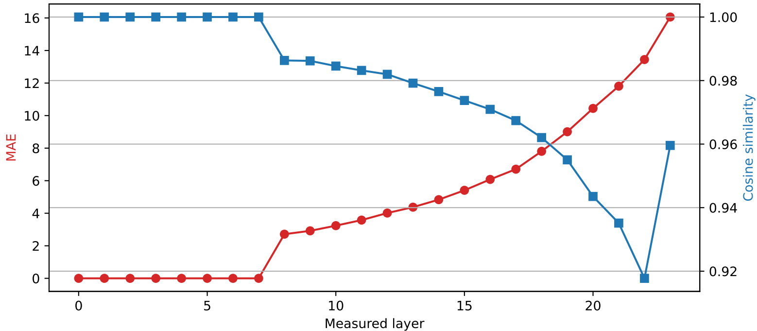
SmolLM2-1.7B-Instruct | Quantized layer 7 | float64 → int4
