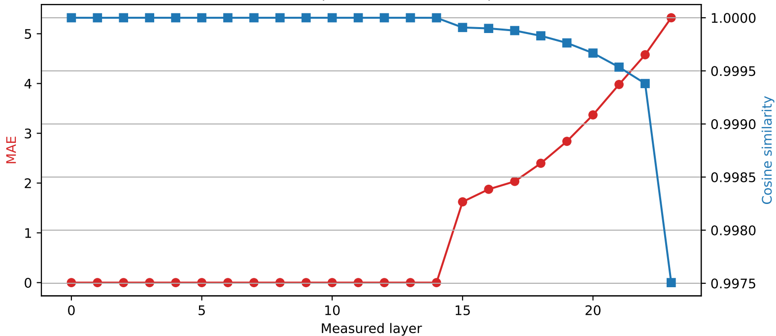
SmolLM2-1.7B-Instruct | Quantized layer 14 | float64 \rightarrow int4
