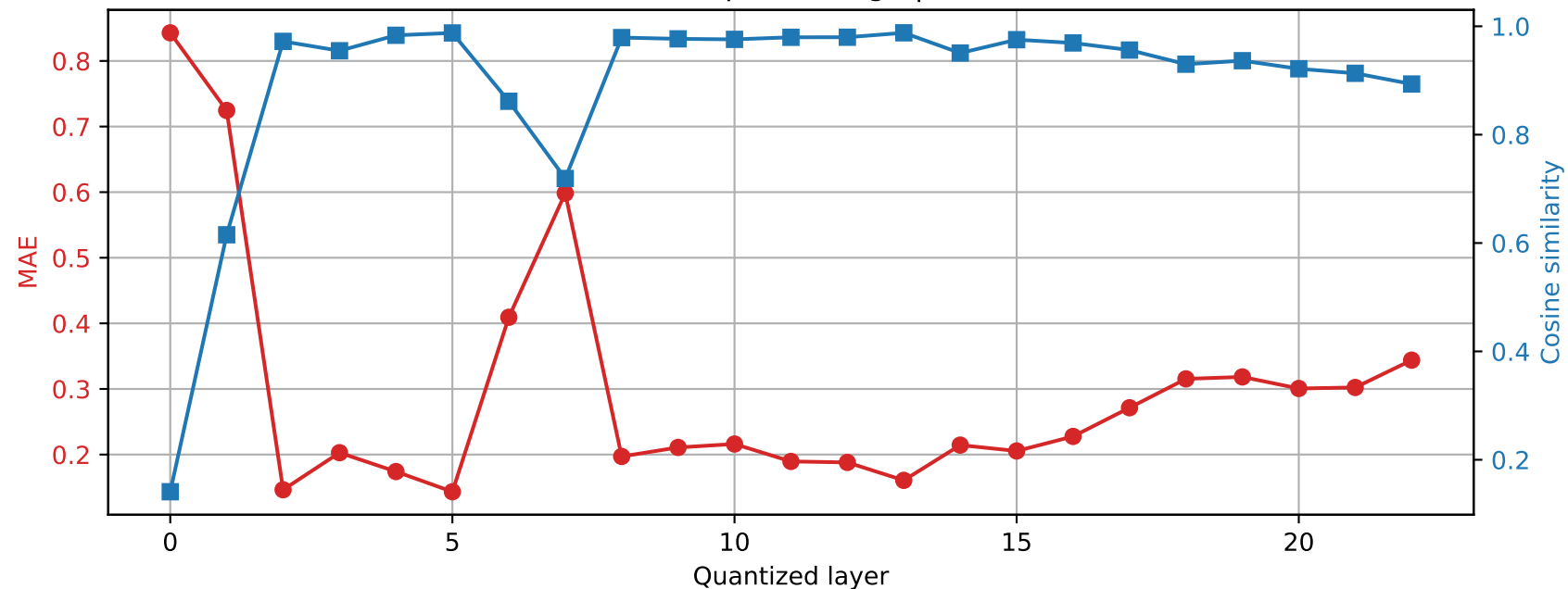
SmolLM2-1.7B-Instruct | Prompt 2 Final RMSNorm output damage | float64 \rightarrow int4
