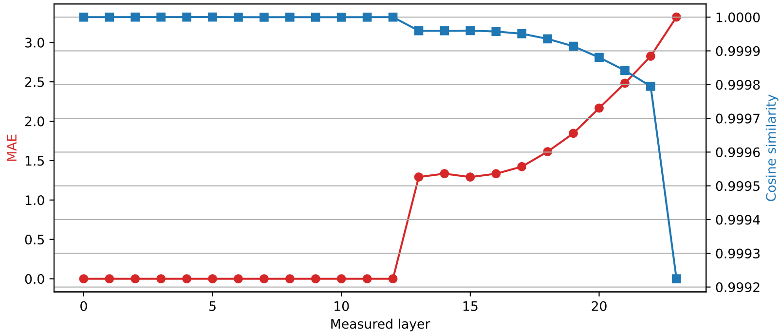
SmolLM2-1.7B-Instruct | Quantized layer 12 | float64 → int4
