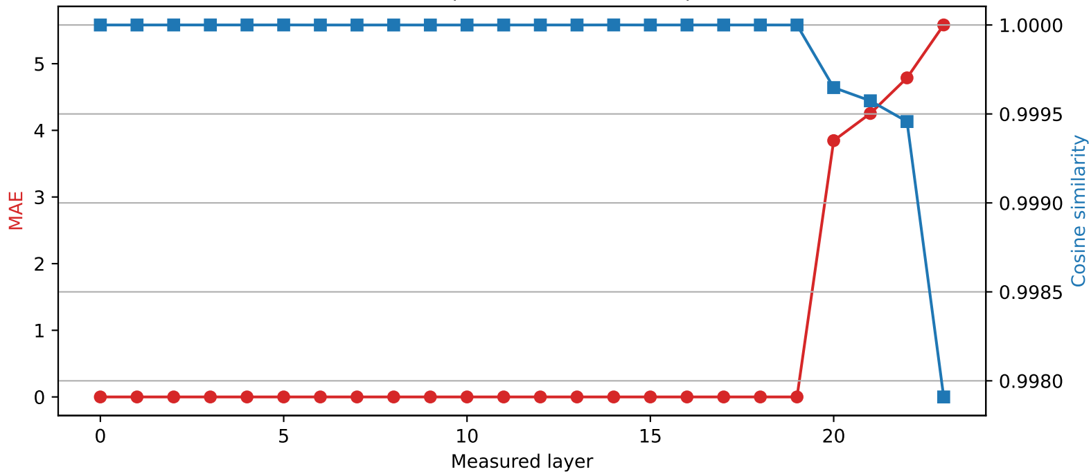
SmolLM2-1.7B-Instruct | Quantized layer 19 | float64 → int4
