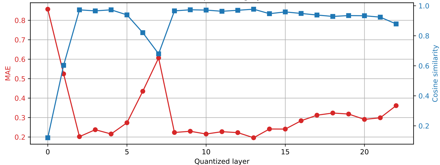
SmolLM2-1.7B-Instruct | Prompt 3 Final RMSNorm output damage | float64 \rightarrow int4
