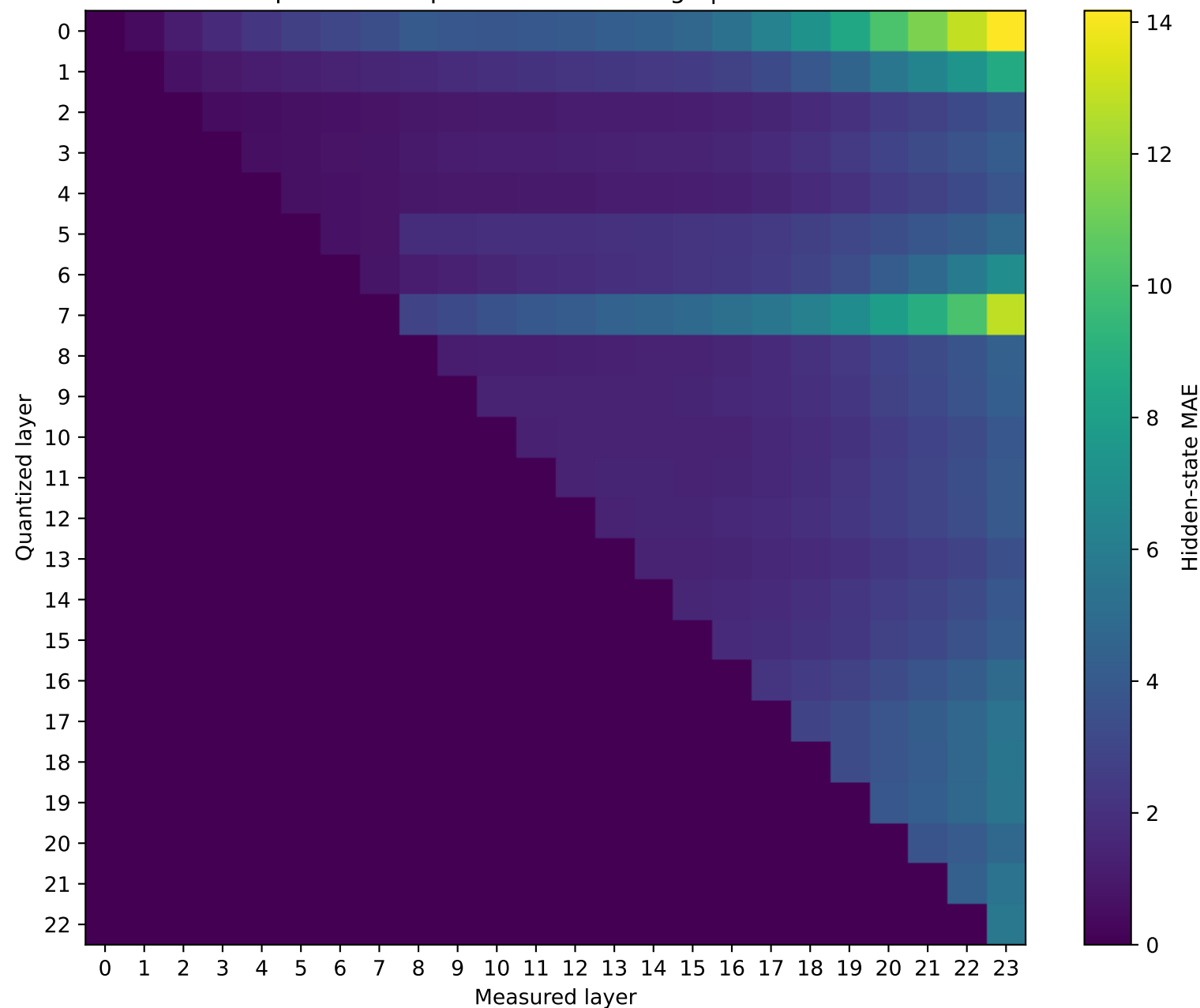
SmolLM2-1.7B-Instruct Prompt 3: MAE representation damage | float64 → int4
