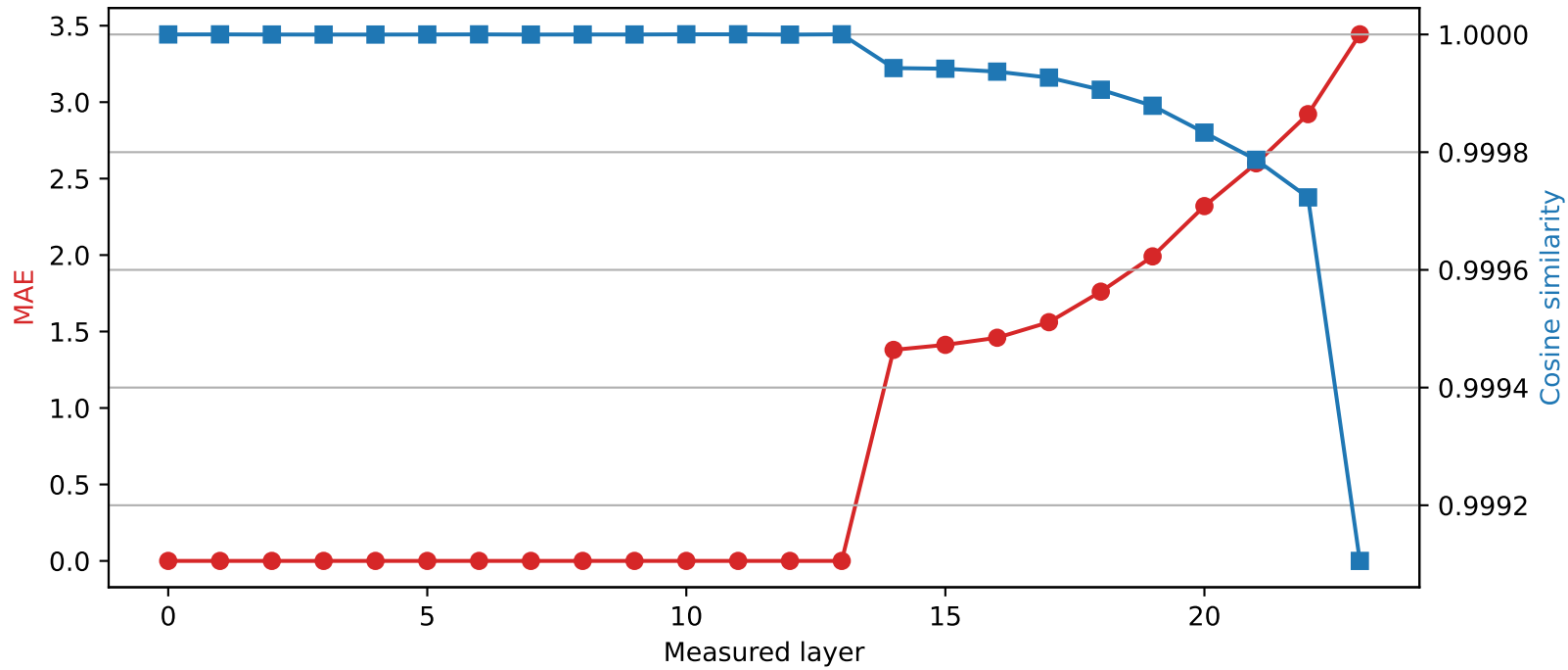
SmolLM2-1.7B-Instruct | Quantized layer 13 | float64 → int4
