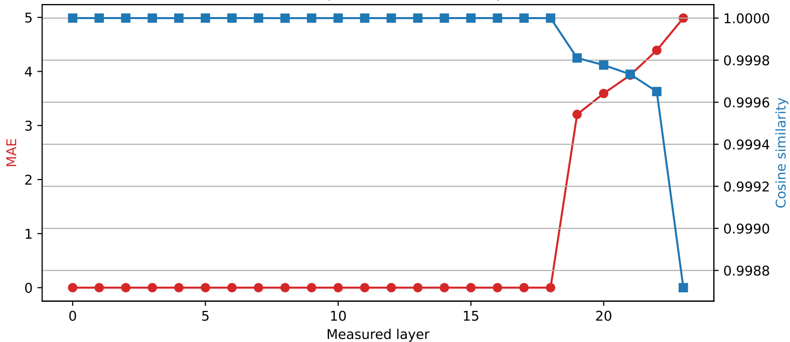
SmolLM2-1.7B-Instruct | Quantized layer 18 | float64 → int4
