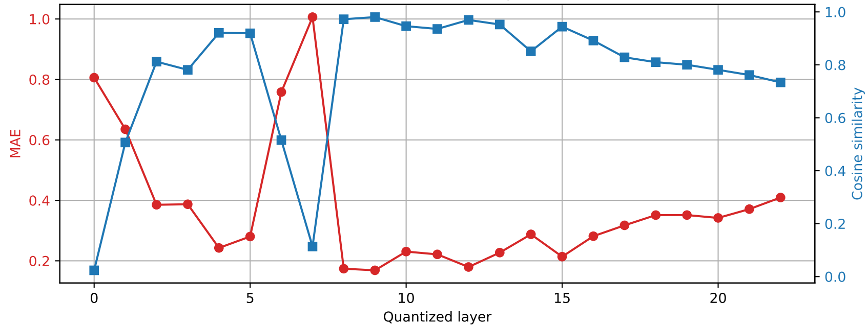
SmolLM2-1.7B-Instruct | Prompt 0 Final RMSNorm output damage | float64 \rightarrow int2
