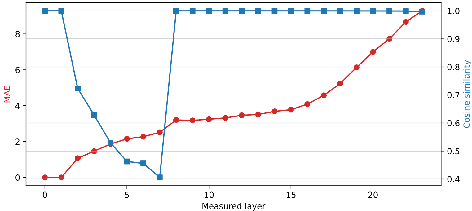
SmolLM2-1.7B-Instruct | Quantized layer 1 | float64 → int2
