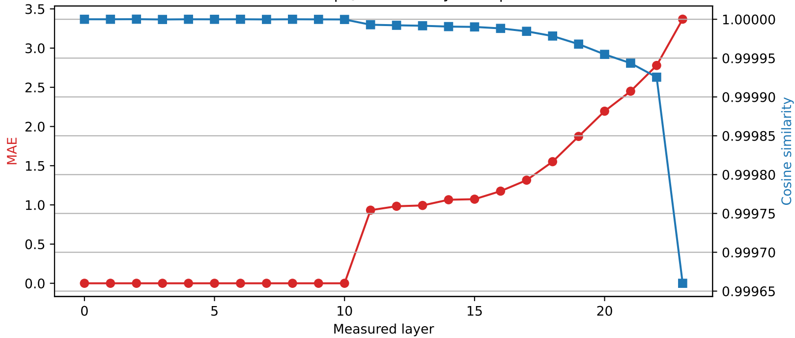
SmolLM2-1.7B-Instruct | Quantized layer 10 | float64 \rightarrow int2
