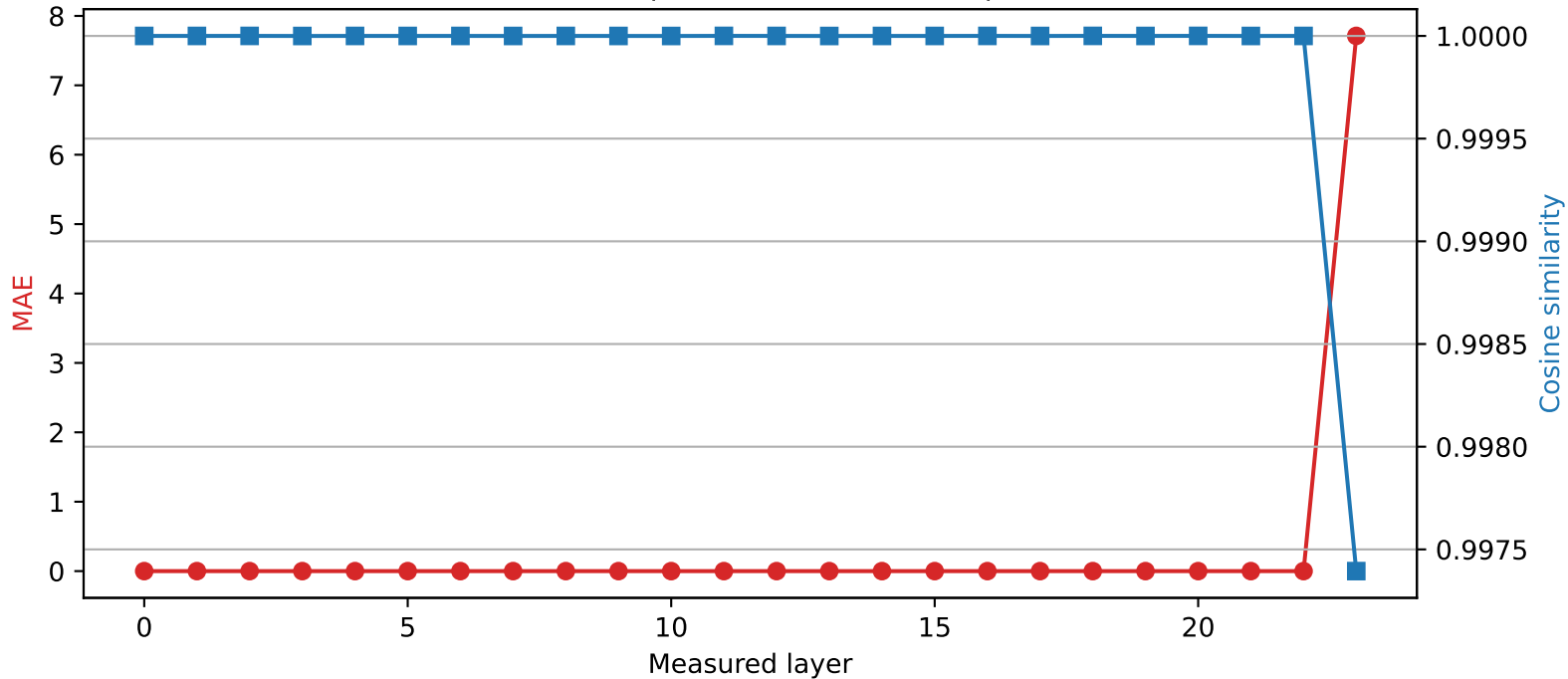
SmolLM2-1.7B-Instruct | Quantized layer 22 | float64 → int2
