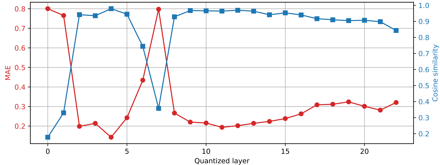
SmolLM2-1.7B-Instruct | Prompt 1 Final RMSNorm output damage | float64 \rightarrow int2
