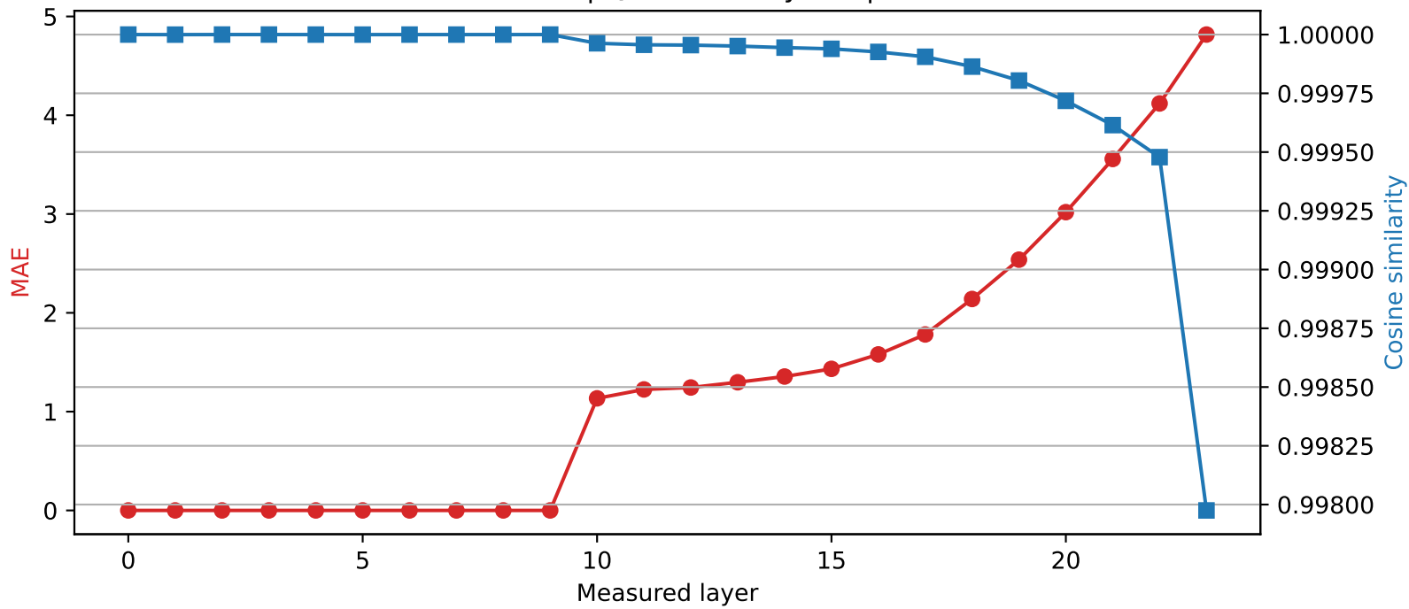
SmolLM2-1.7B-Instruct | Quantized layer 9 | float64 → int2
