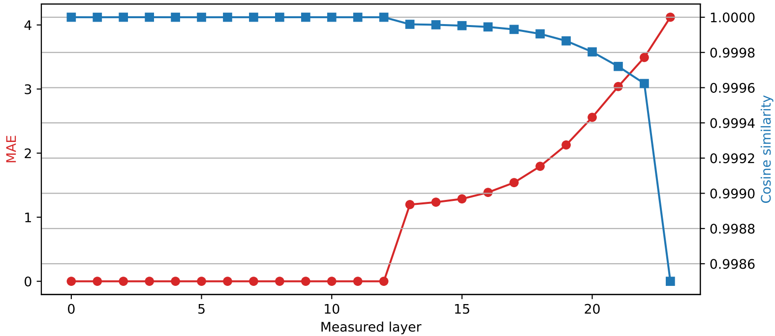
SmolLM2-1.7B-Instruct | Quantized layer 12 | float64 → int2
