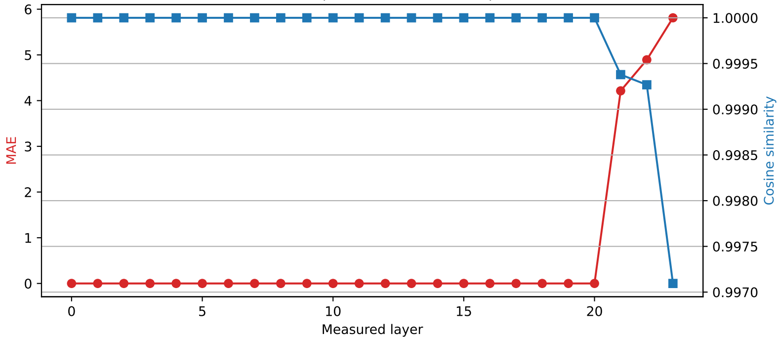
SmolLM2-1.7B-Instruct | Quantized layer 20 | float64 → int2
