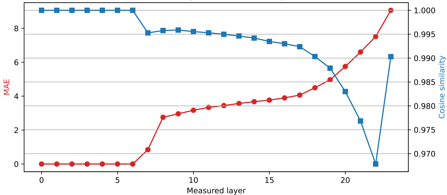
SmolLM2-1.7B-Instruct | Quantized layer 6 | float64 → int2
