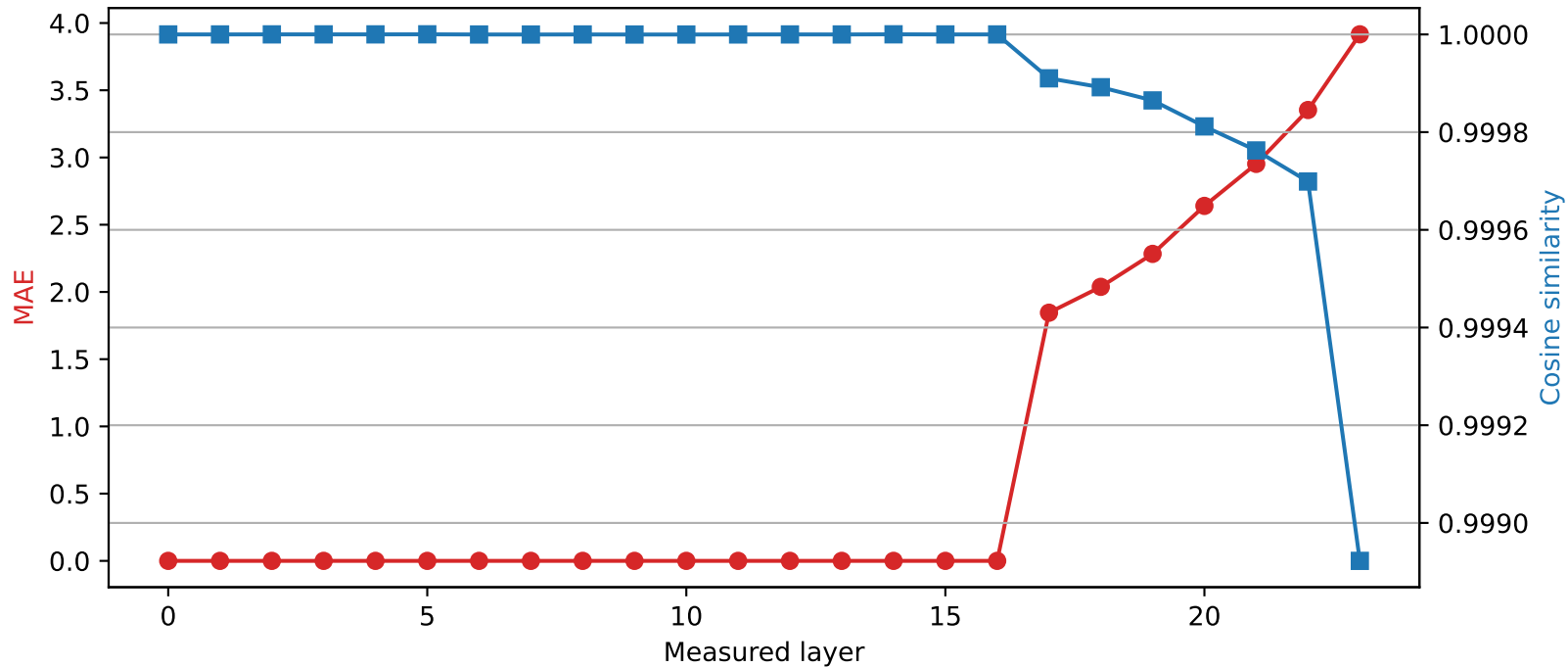
SmolLM2-1.7B-Instruct | Quantized layer 16 | float64 → int2
