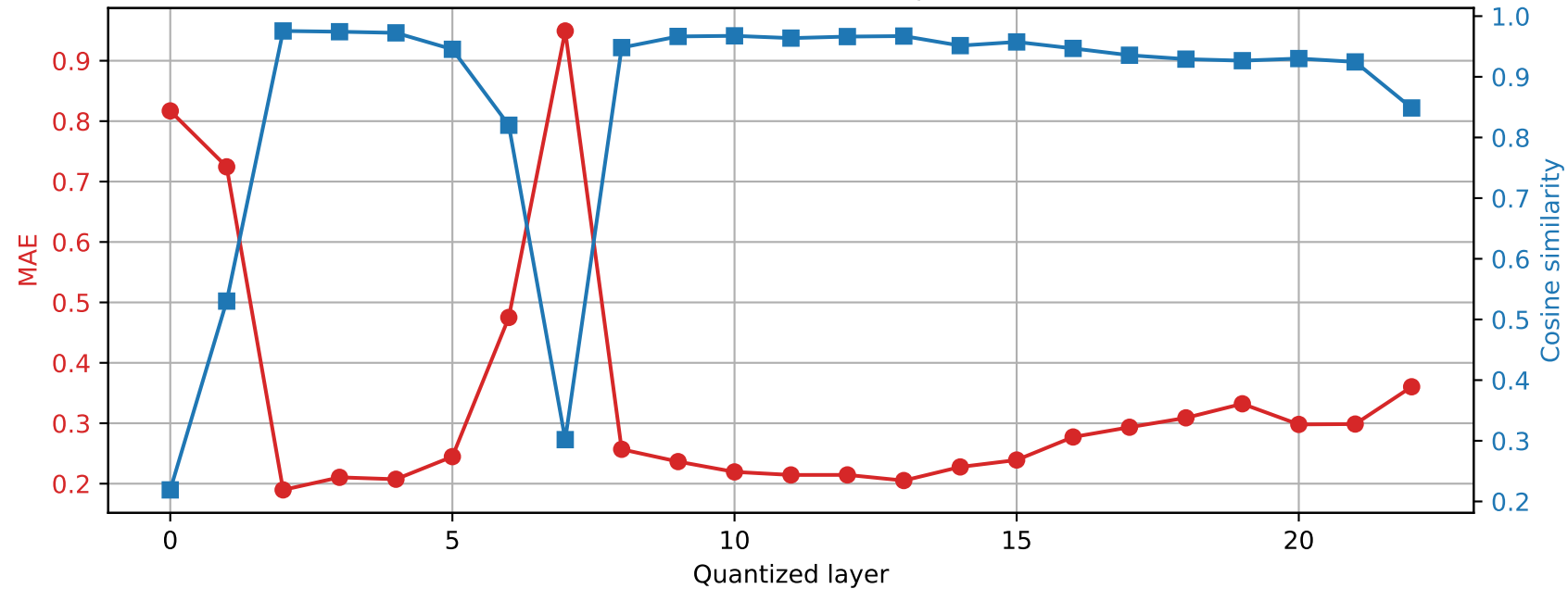
SmolLM2-1.7B-Instruct | Prompt 3 Final RMSNorm output damage | float64 \rightarrow int2
