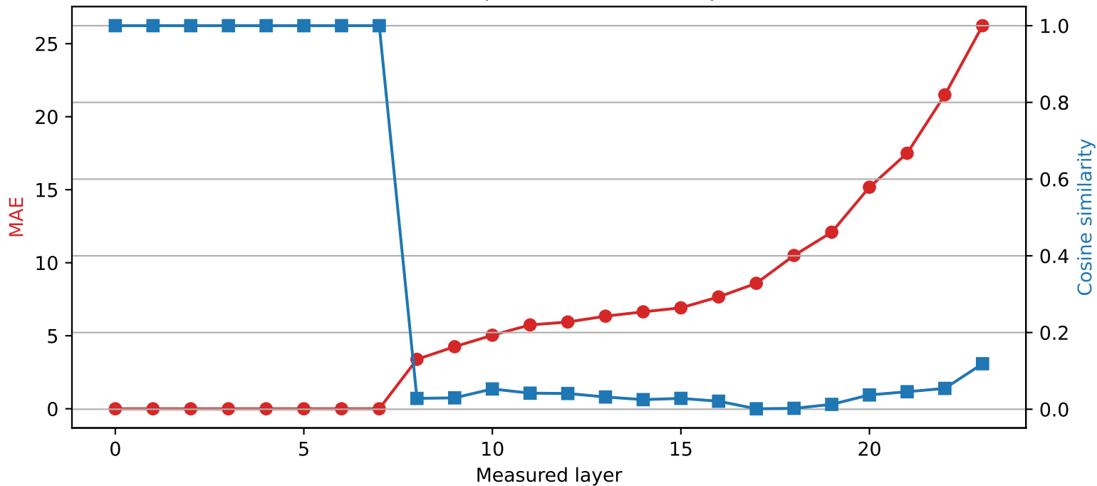
SmolLM2-1.7B-Instruct | Quantized layer 7 | float64 → int2
