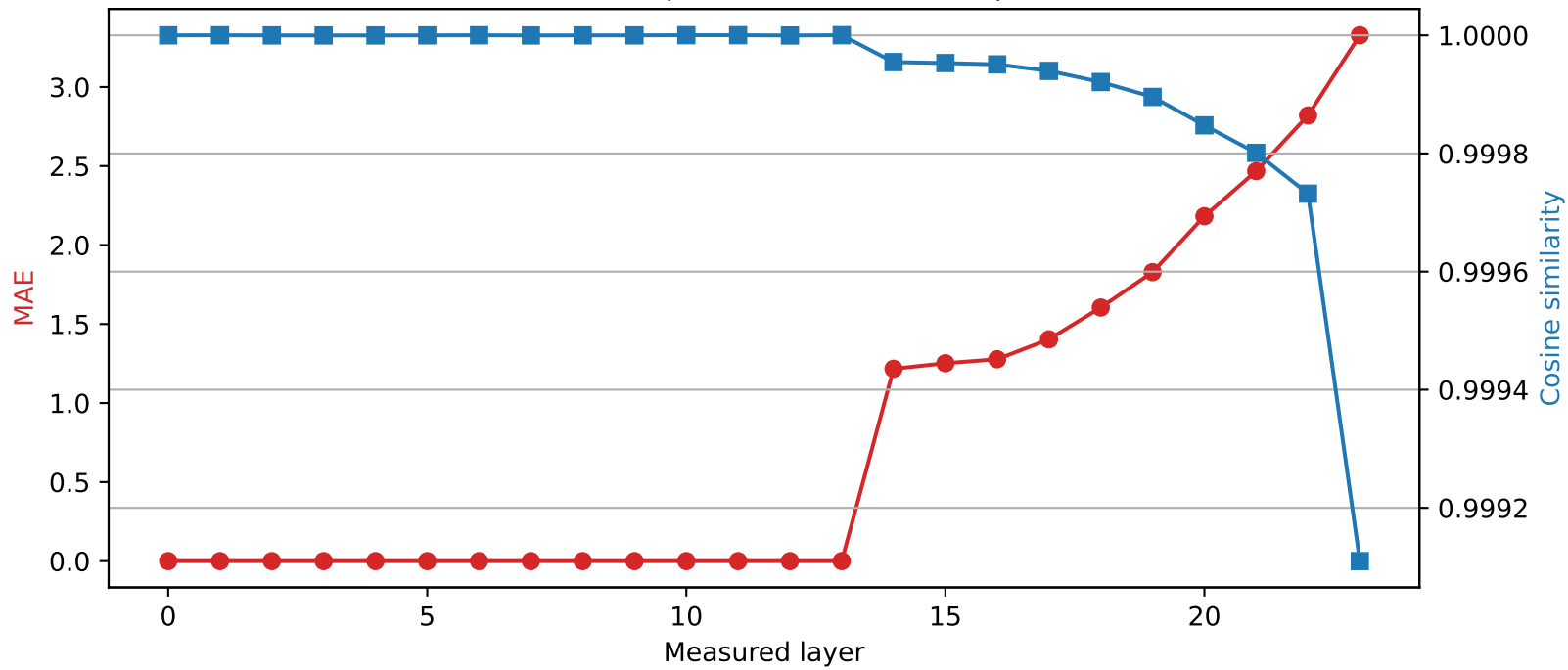
SmolLM2-1.7B-Instruct | Quantized layer 13 | float64 → int2
