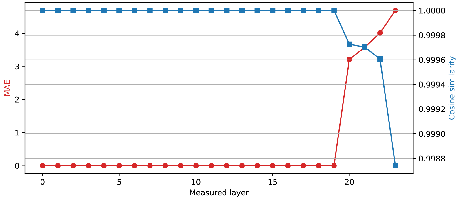
SmolLM2-1.7B-Instruct | Quantized layer 19 | float64 → int2
