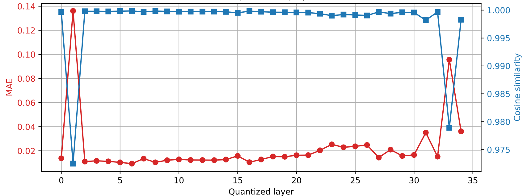
SmolLM3-3B | Prompt 0 Final RMSNorm output damage | float16 \rightarrow int8
