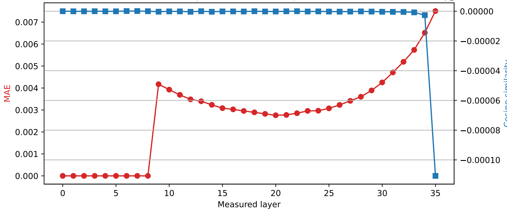
SmolLM3-3B | Quantized layer 8 | float16 → int8
