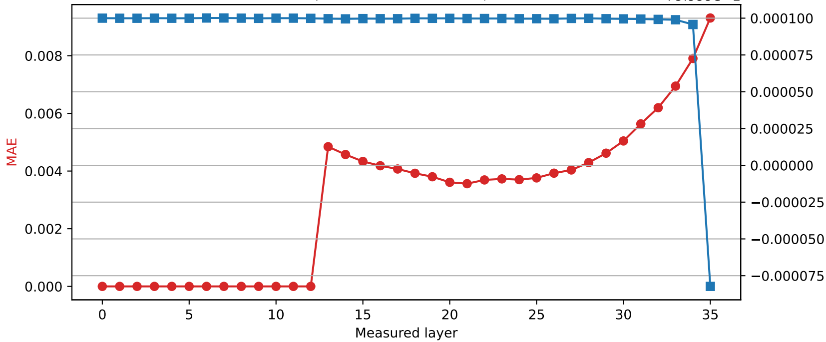
SmolLM3-3B | Quantized layer 12 | float16 → int8
