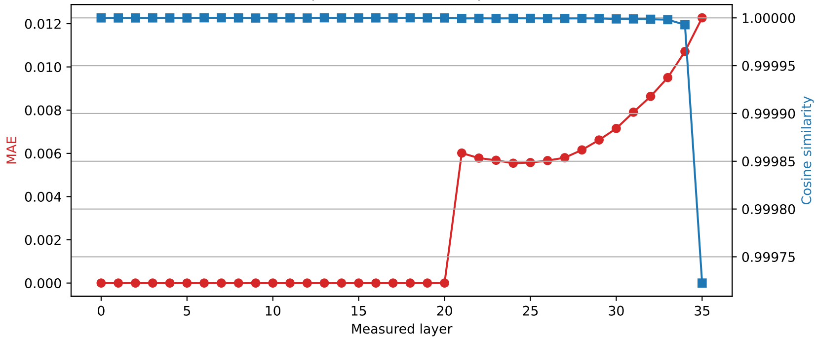
SmolLM3-3B | Quantized layer 20 | float16 \rightarrow int8
