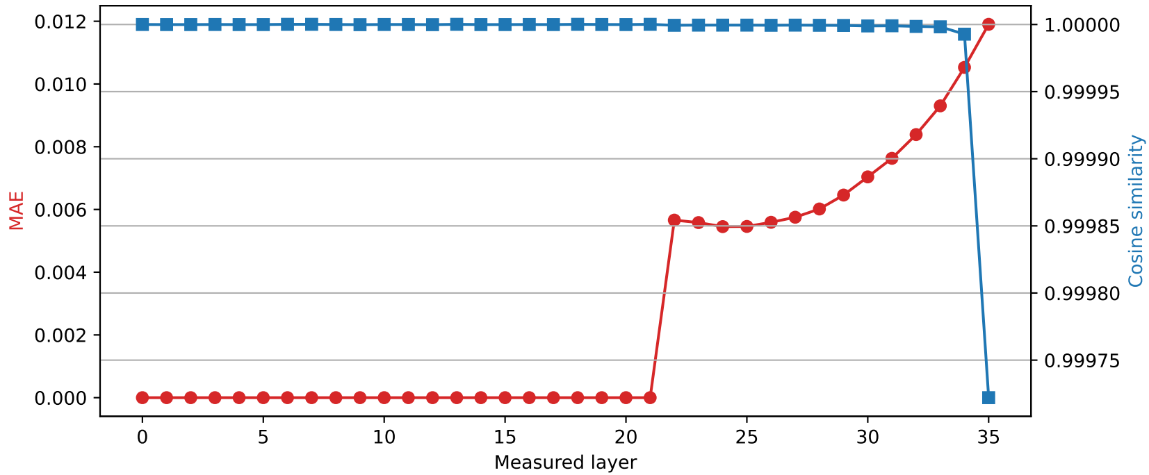
SmolLM3-3B | Quantized layer 21 | float16 → int8
