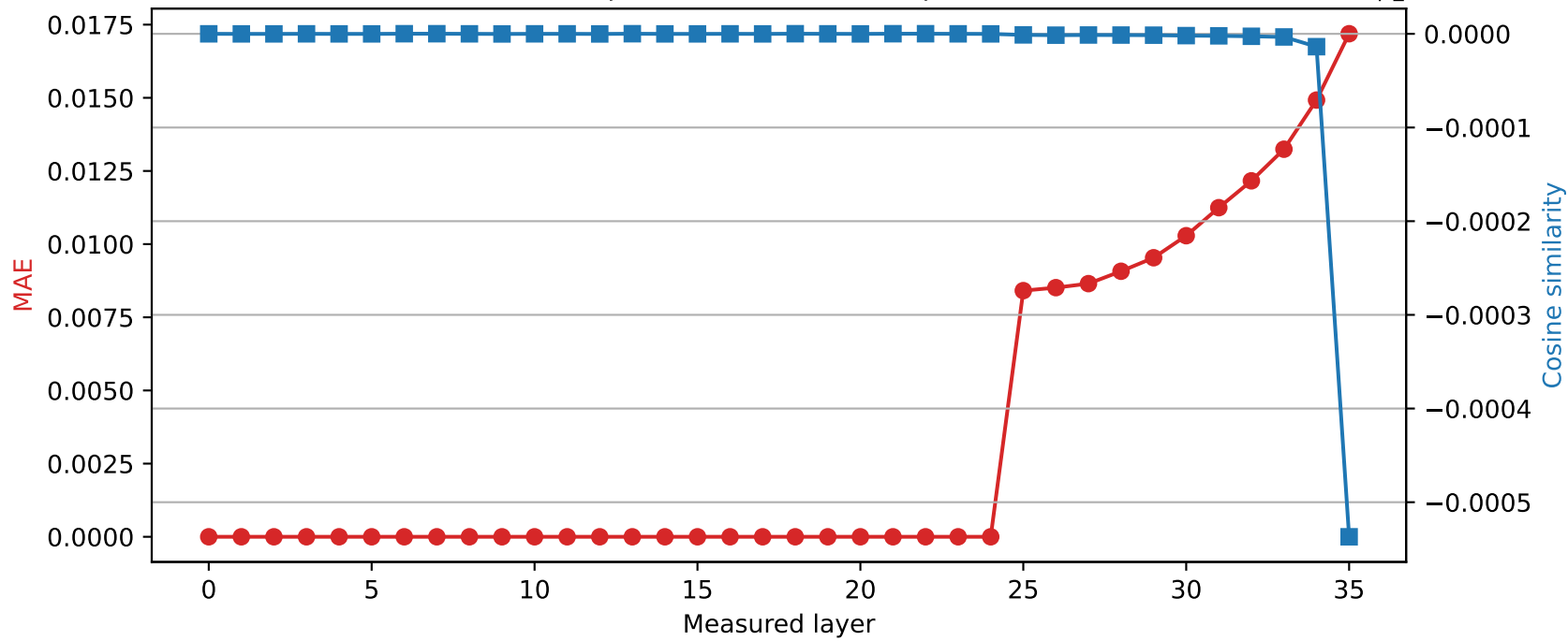
SmolLM3-3B | Quantized layer 24 | float16 \rightarrow int8
