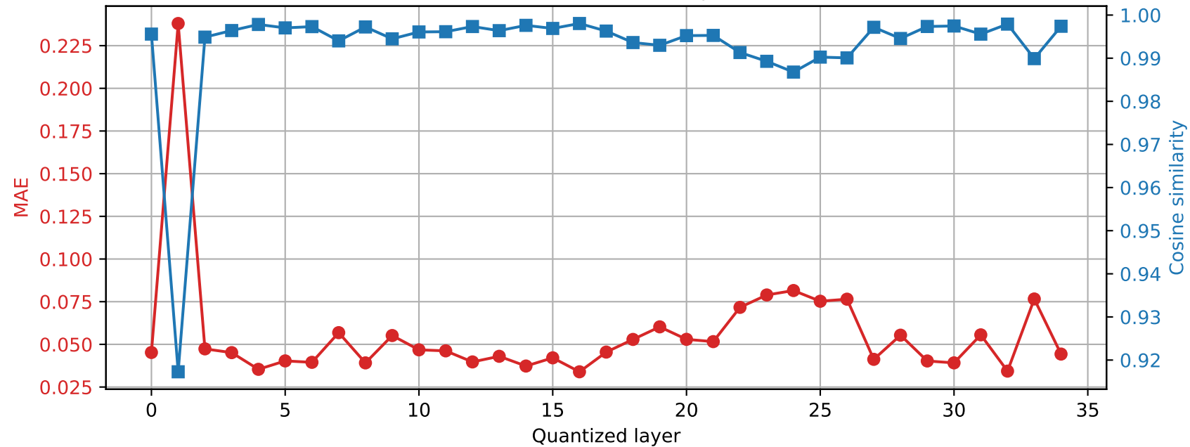
SmolLM3-3B | Prompt 1 Final RMSNorm output damage | float16 \rightarrow int8
