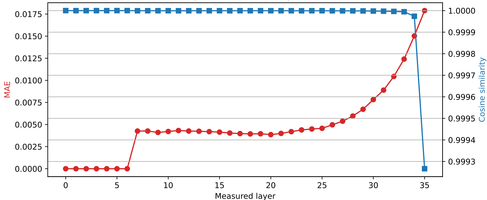
SmolLM3-3B | Quantized layer 6 | float16 \rightarrow int8
