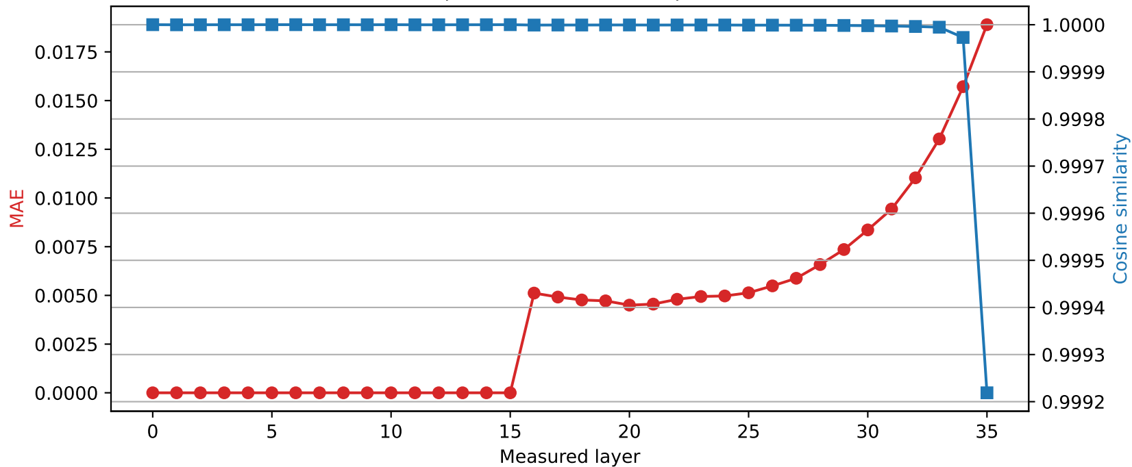
SmolLM3-3B | Quantized layer 15 | float16 \rightarrow int8
