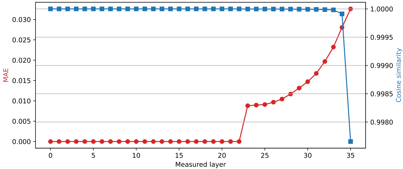
SmolLM3-3B | Quantized layer 22 | float16 \rightarrow int8
