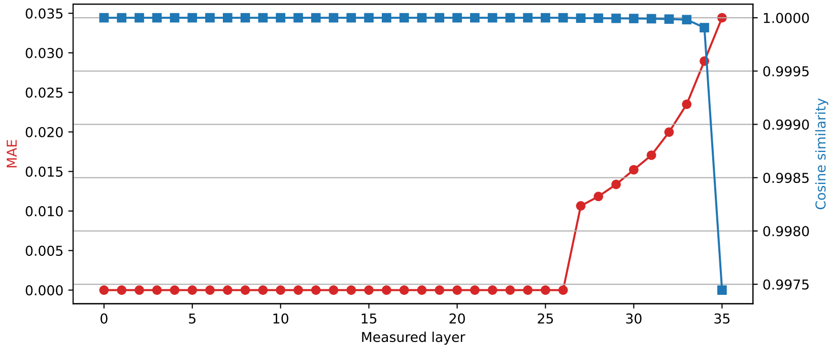
SmolLM3-3B | Quantized layer 26 | float16 \rightarrow int8
