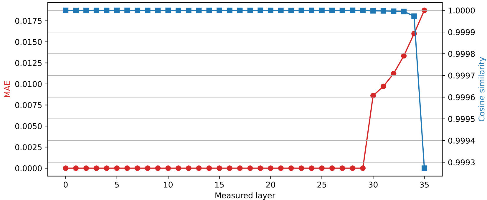
SmolLM3-3B | Quantized layer 29 | float16 \rightarrow int8
