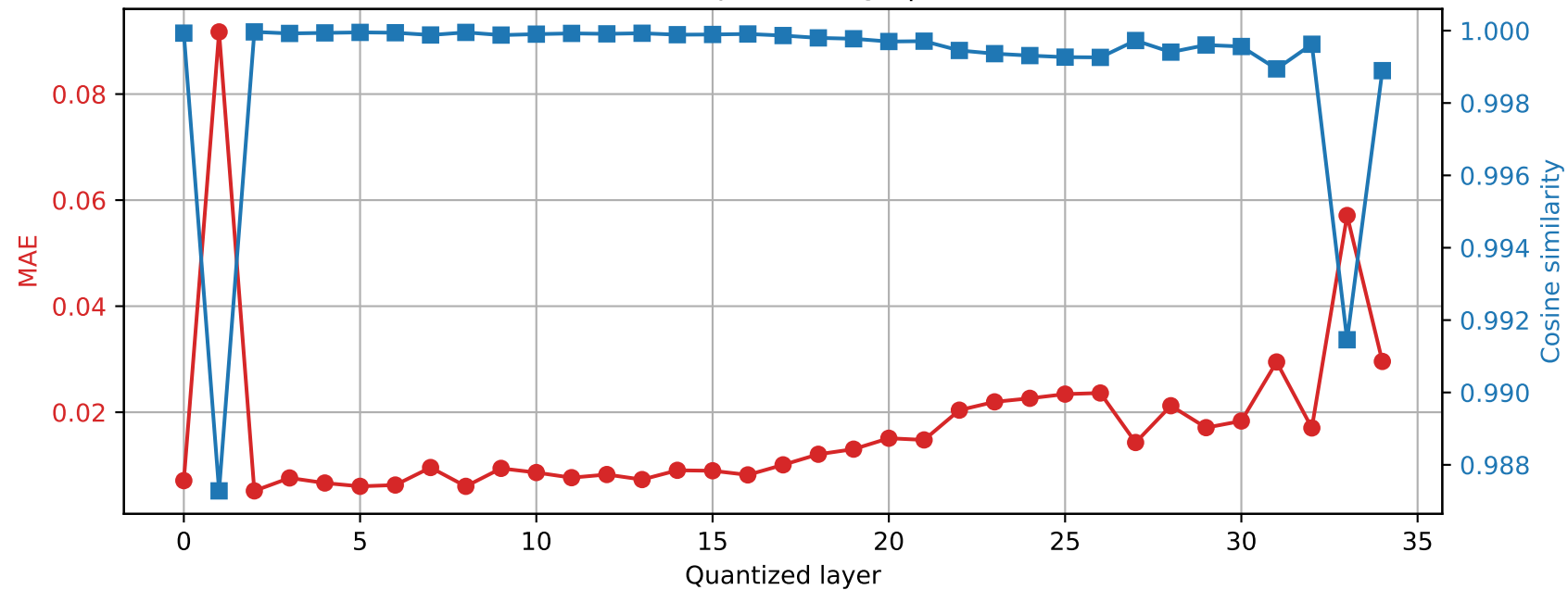
SmolLM3-3B | Prompt 2 Final RMSNorm output damage | float16 \rightarrow int8
