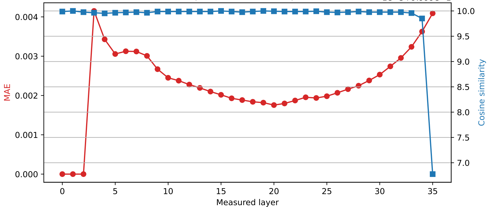
SmolLM3-3B | Quantized layer 2 | float16 → int8
