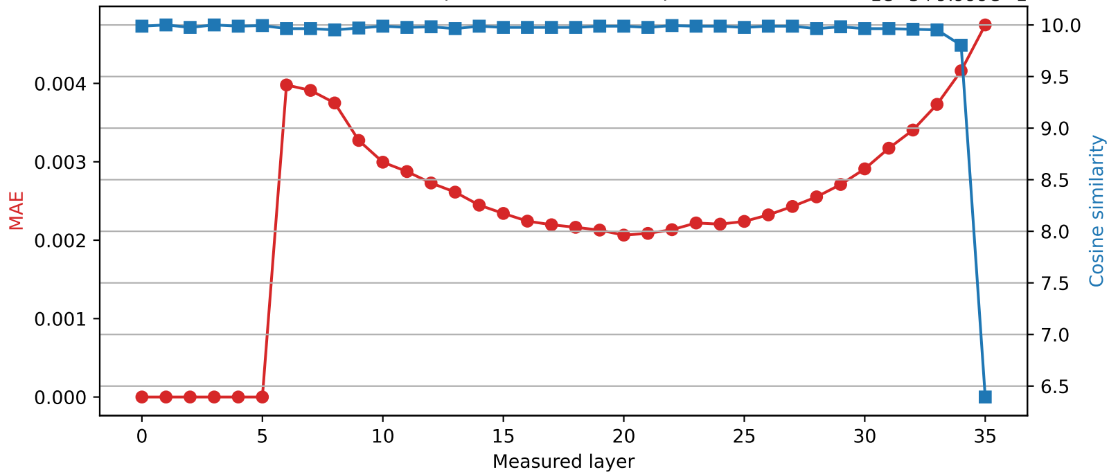
SmolLM3-3B | Quantized layer 5 | float16 → int8
