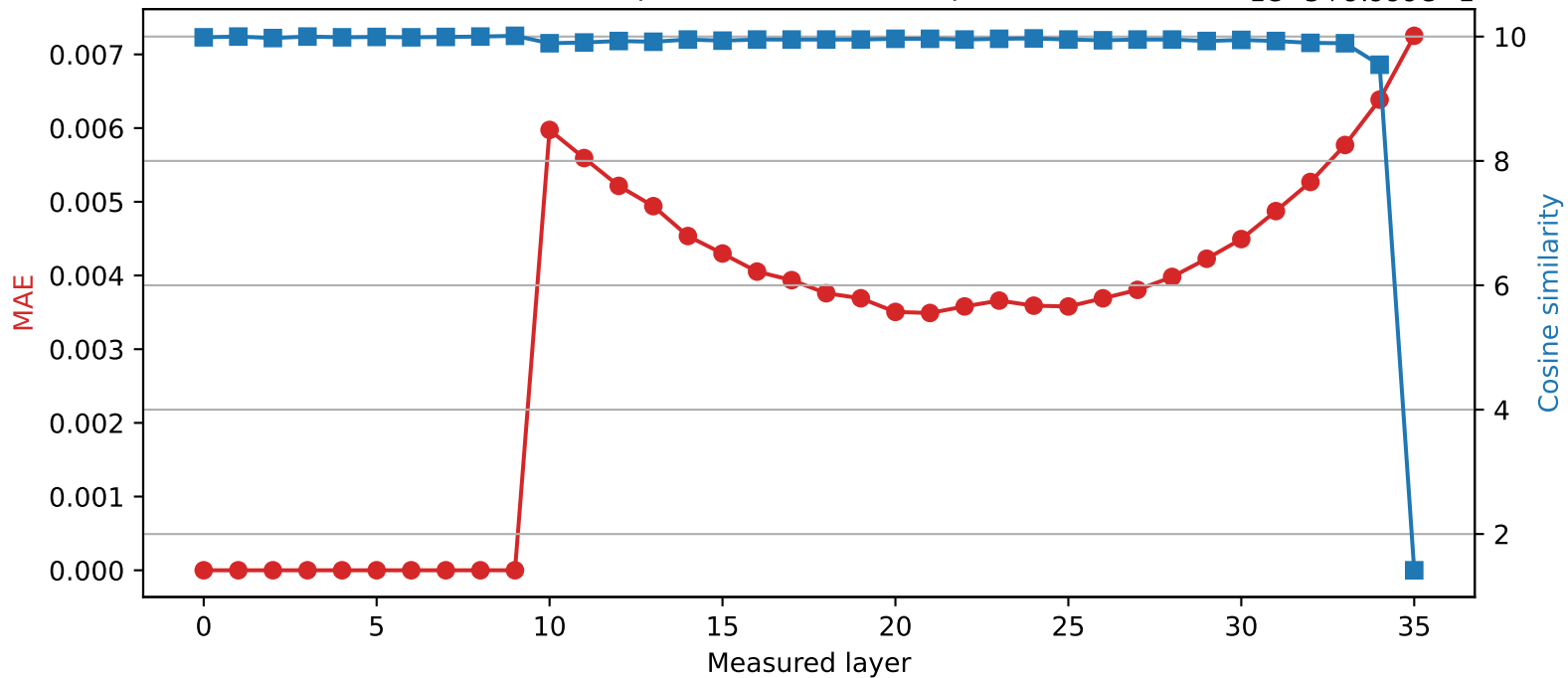
SmolLM3-3B | Quantized layer 9 | float16 → int8
