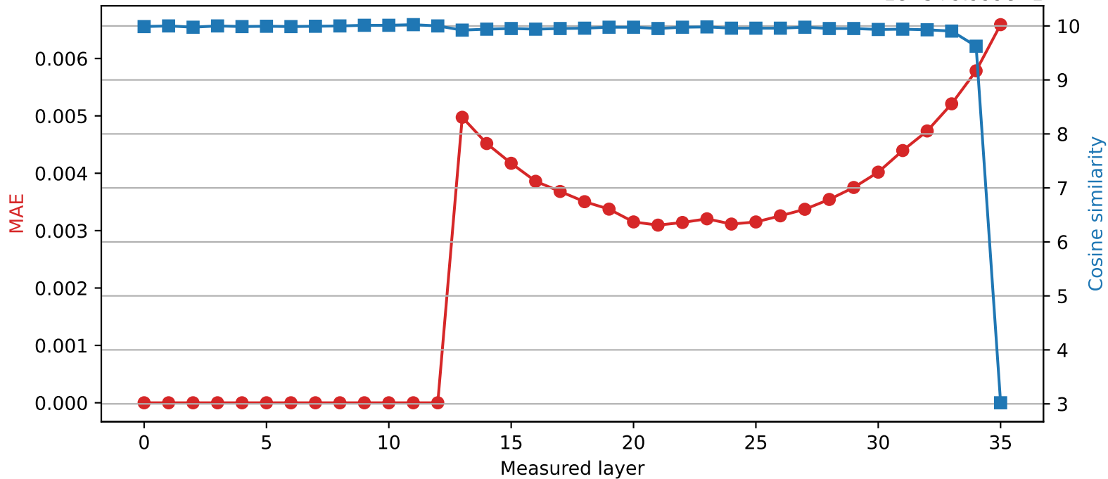
SmolLM3-3B | Quantized layer 12 | float16 → int8
